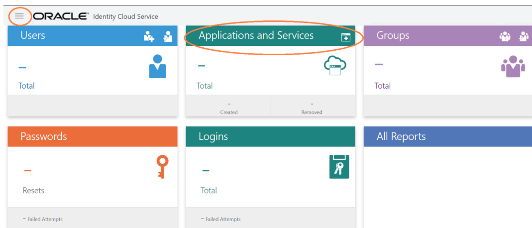
Figure 2-1 Dashboard
