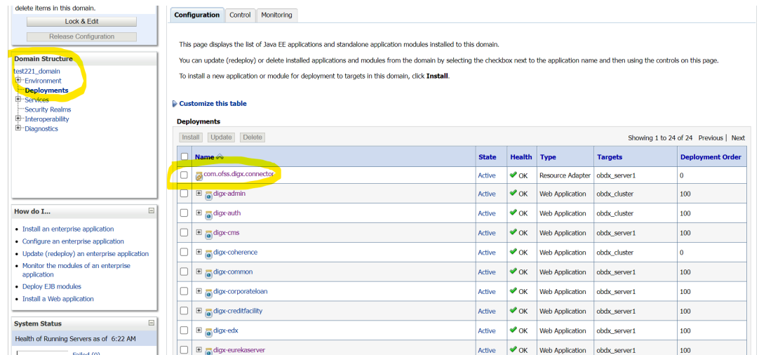
Figure 2-44 Deployments
