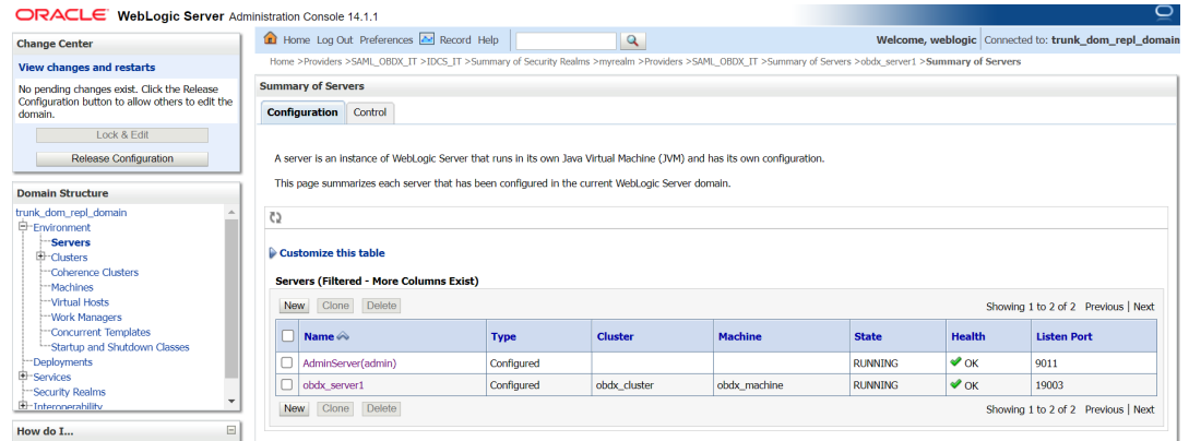
Figure 2-17 Servers
