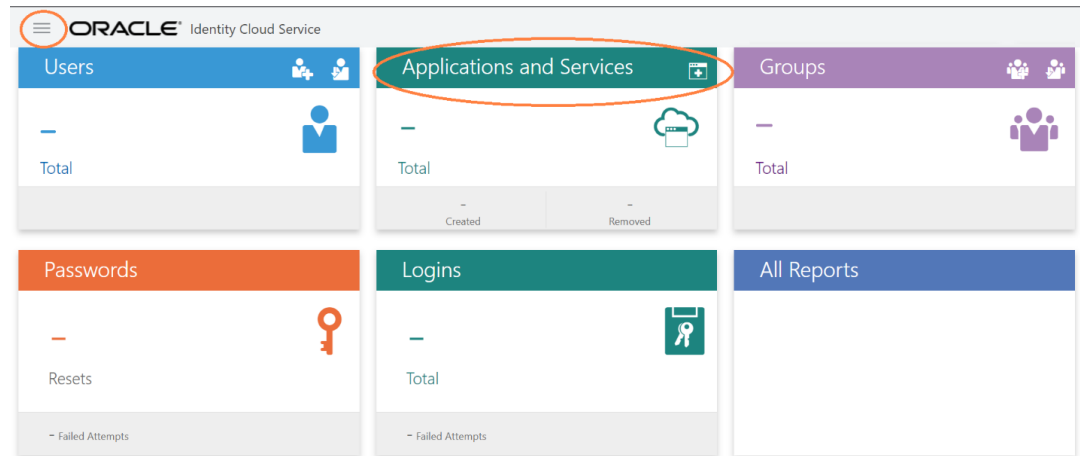
Figure 2-26 Dashboard
