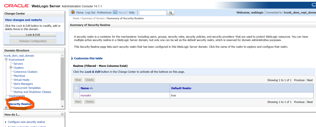
Figure 2-19 Security Realms
