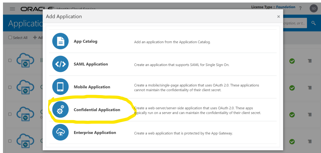
Figure 2-27 Add Application
