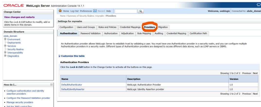
Figure 2-20 Providers
